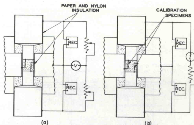
Fig. 2 Methods used for monitoring transitions for two independent circuits
