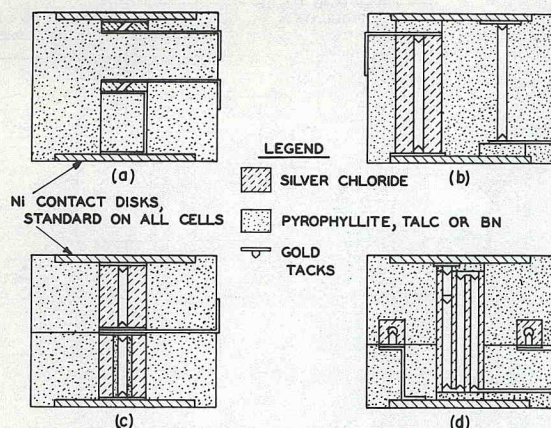
Fig. 3 Cell configuration. Sample size - 0.500-in. dia x 0.400-in. high
