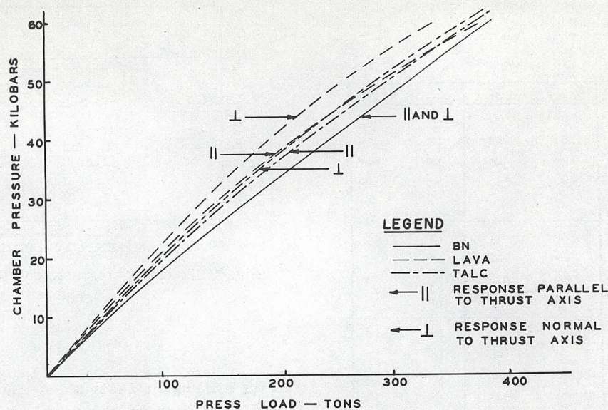
Fig. 7 Calibration curves for selected pyrophyllite, talc, and hot-pressed BN samples. Numerical data given in Table 3
