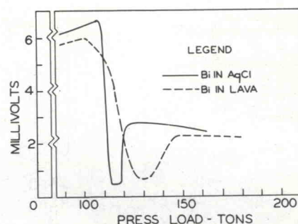
Fig.4 Comparison of response of Bi I-II and II-III transitions in jacketed and un-jacketed samples
