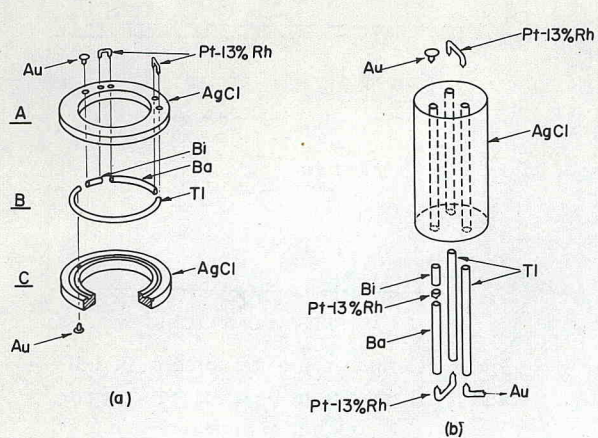
Fig. 5 Exploded views of Bi-Tl-Ba calibration-cell construction
