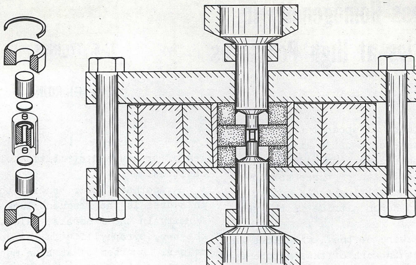
Fig. 1 Cross-sectional view of apparatus
