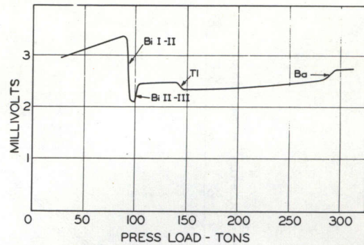
Fig.6 Tracing of response obtained from Bi-Tl-Ba cell
